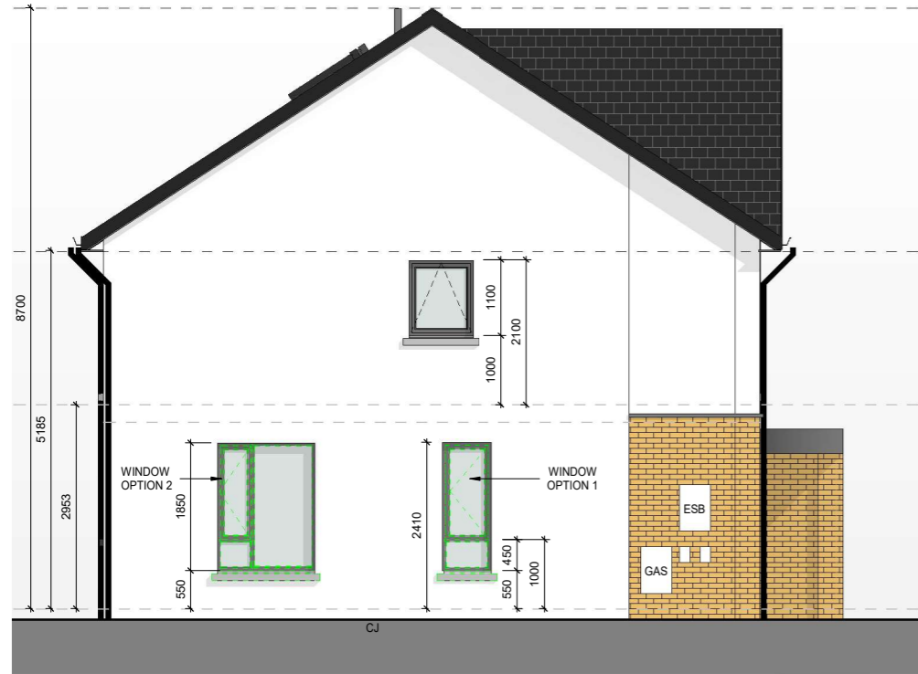
SIDE ELEVATION TYPE D 1: 50 @ A1 1:100 @ A3
