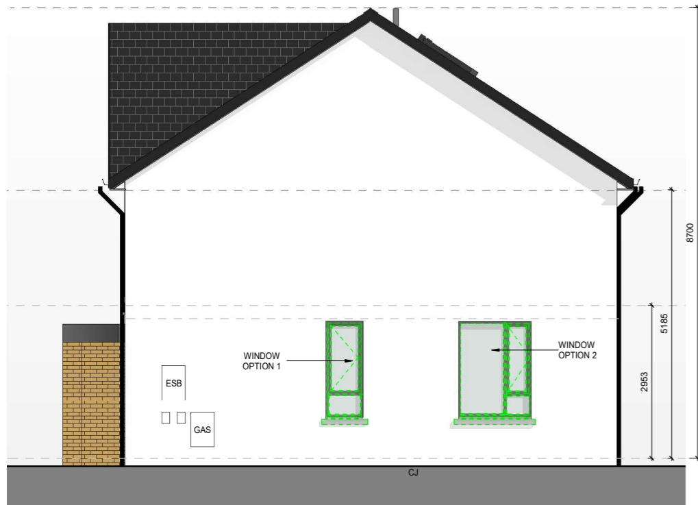
SIDE ELEVATION TYPE D(m) 1: 50 @ A1 1:100 @ A3
