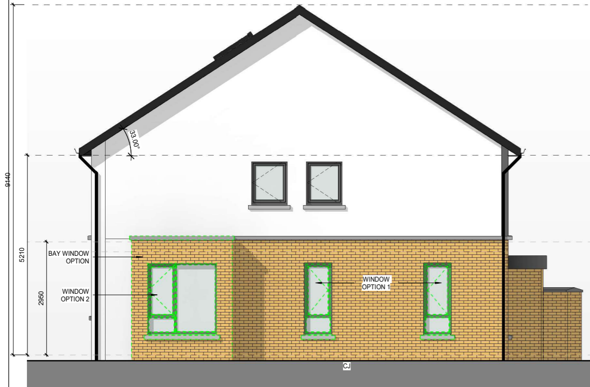
SIDE ELEVATION TYPE E1 1: 50 @ A1 1:100 @ A3
