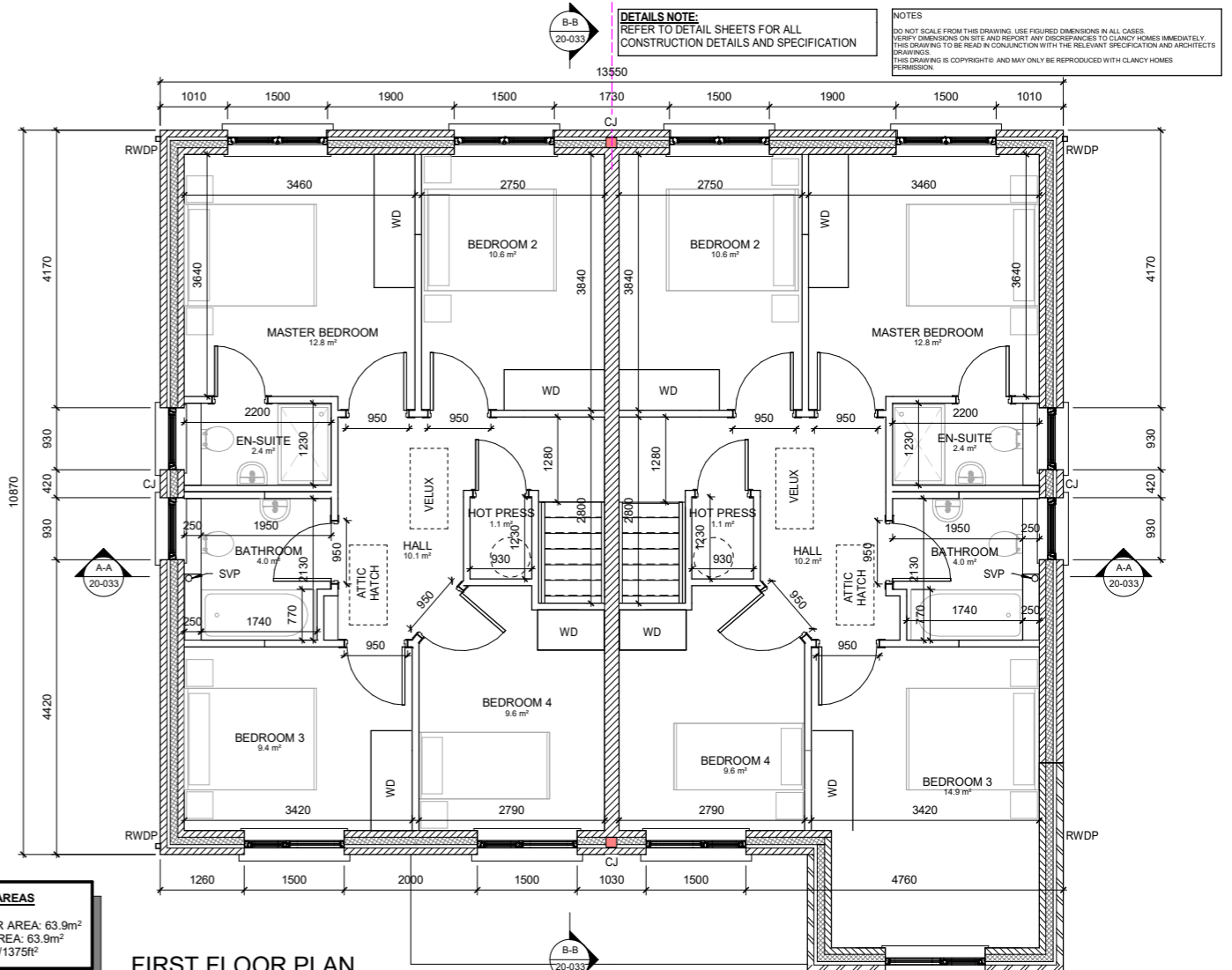
FIRST FLOOR PLAN TYPE F1 1:50 @ A1 1:100 @ A3
