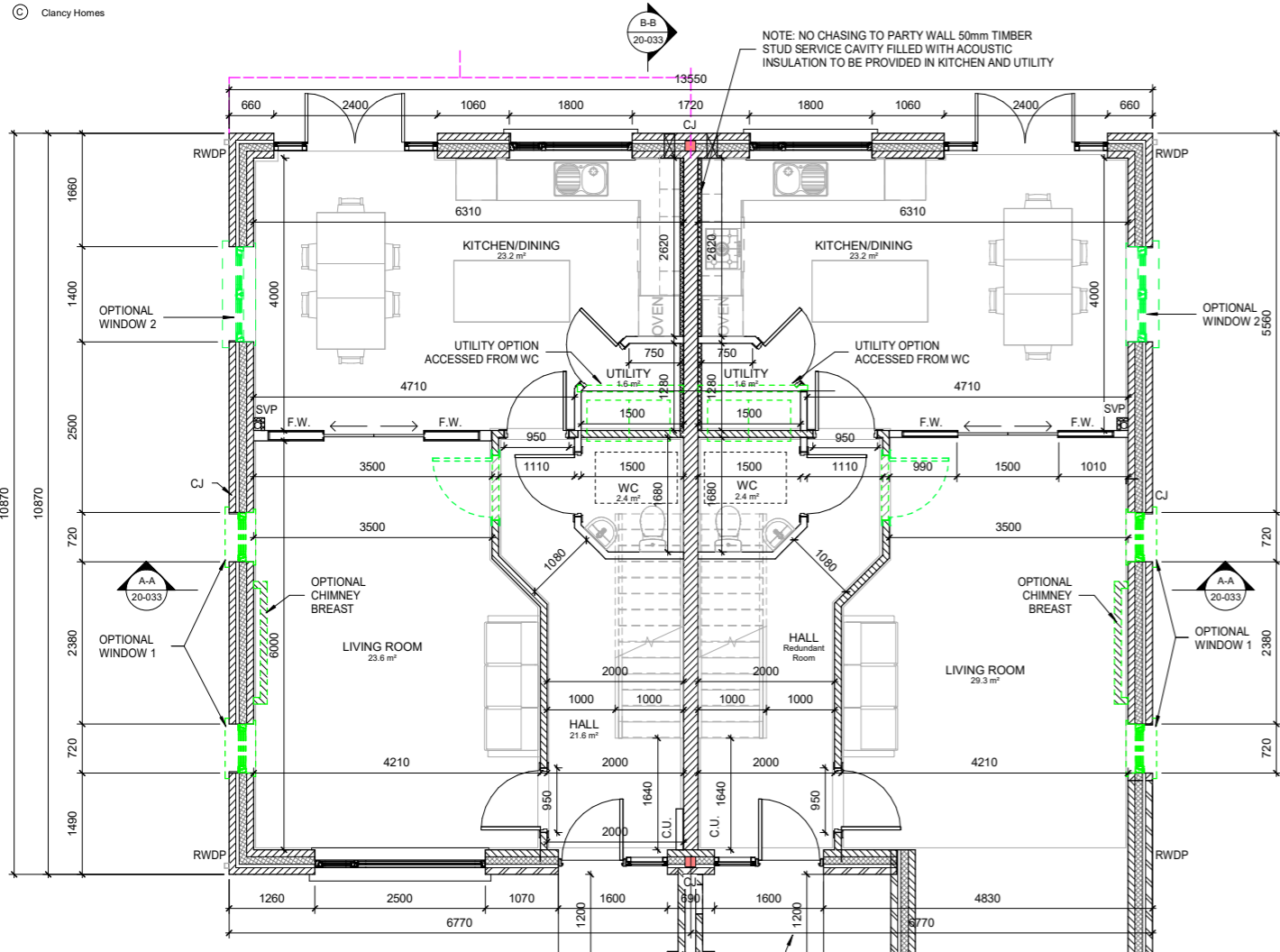
GROUND FLOOR PLAN TYPE F2 1: 50 @ A1 1:100 @ A3
