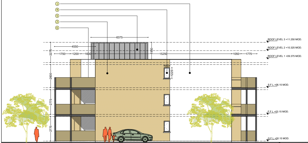
APARTMENT BLOCK - TYPE 'A' NORTH (SIDE) ELEVATION SCALE 1:200 @A3, 1:100@A1
