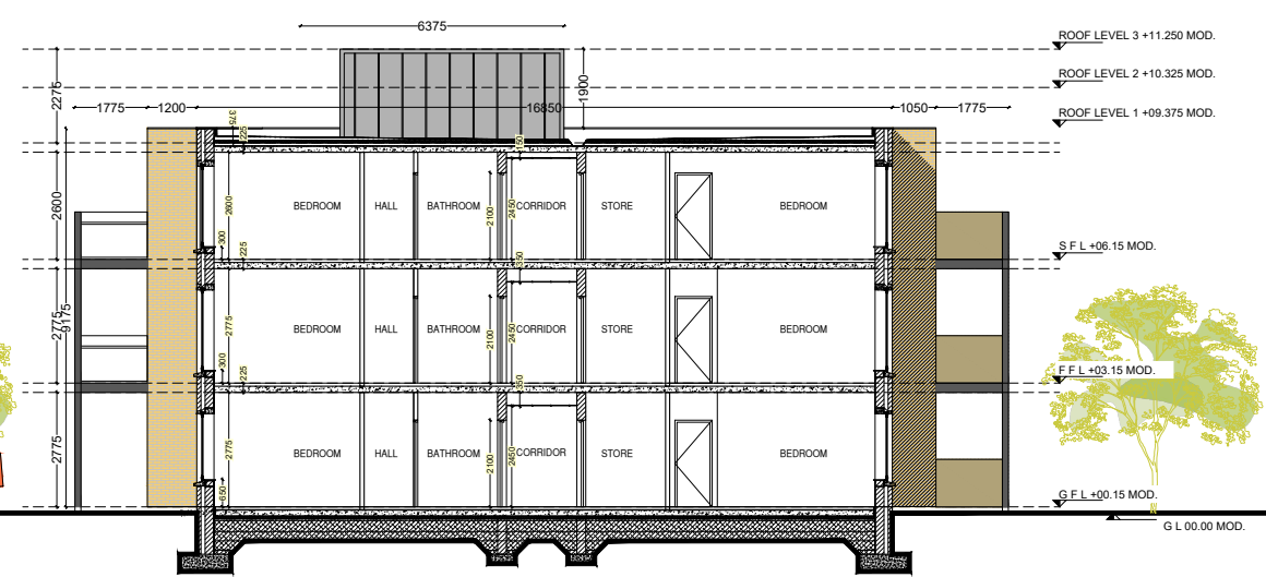
APARTMENT BLOCK - TYPE 'A' TYPICAL SECTION SCALE 1:200 @A3, 1:100@A1
