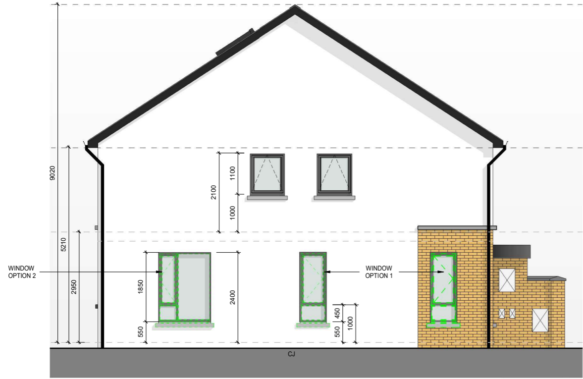
SIDE ELEVATION TYPE A(m) 1: 50 @ A1 1:100 @ A3
