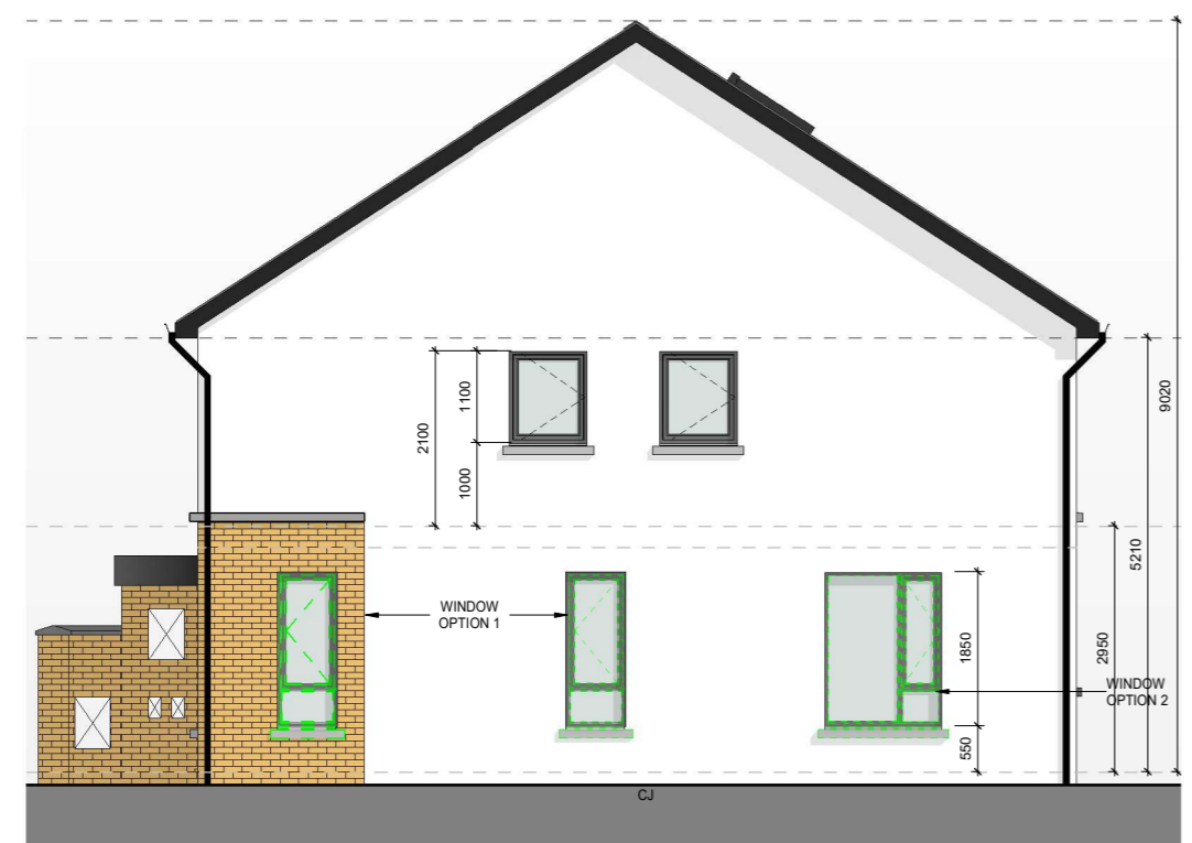
SIDE ELEVATION TYPE A 1: 50 @ A1 1:100 @ A3
