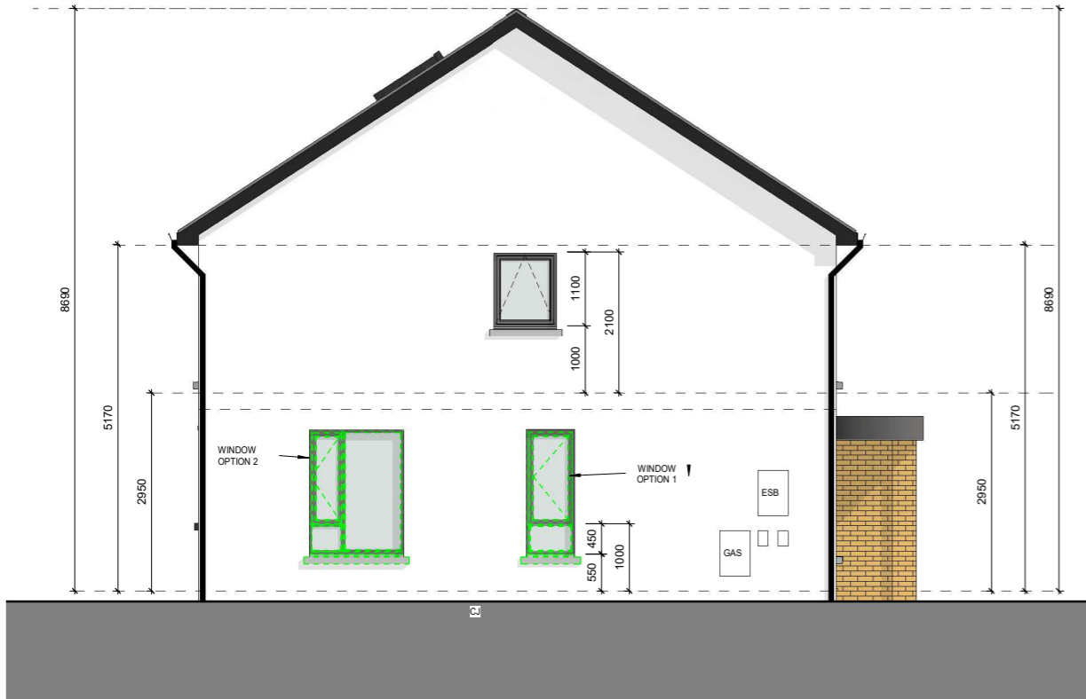
SIDE ELEVATION Type B(m)1 1: 50 @ A1 1:100 @ A3
