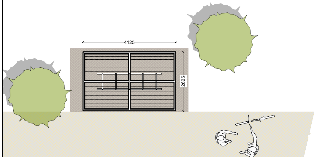
TYPICAL BICYCLE SHELTER PLAN
