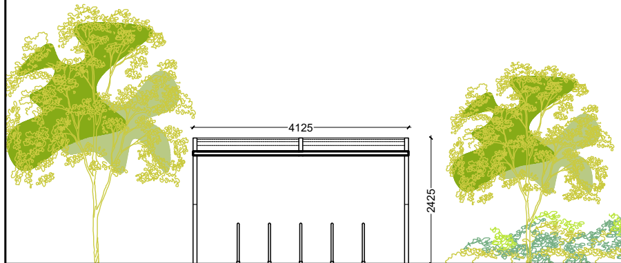
BICYCLE SHELTER LONG ELEVATION
