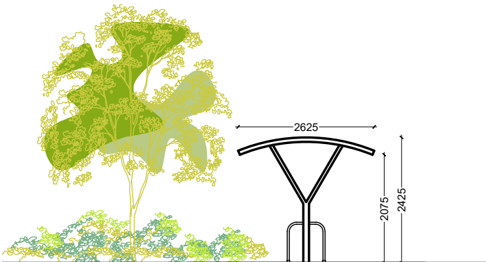
BICYCLE SHELTER SHORT ELEVATION
